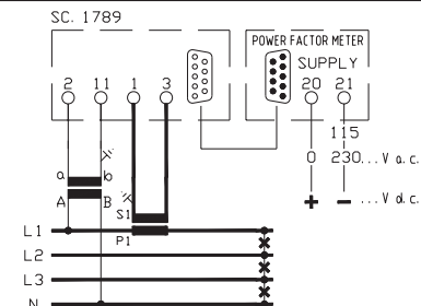
A96PNL - A14PNL trifase 4 fili carico equilibrato 3 phase 4 wires balanced load
