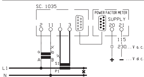
A96PSL - A14PSL monofase - single-phase
