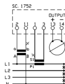
MCO...WXXXXA A/F48WN - A/F48PN - A/F52WN A/F72WN - A/F96WN - A/F14WN trifase 4 fili carico equilibrato 3 phase 4 wires balanced load
