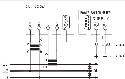
A96PYL - A14PYL trifase 3 fili carico equilibrato 3 phase 3 wires balanced load
